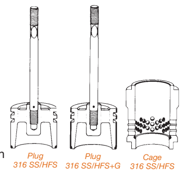
Figure 13. Hard Facing
