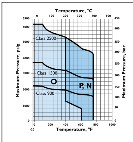
Figure 10. Trim Chart For Stainless Steel Body (ASTM A 351, CF8M)
